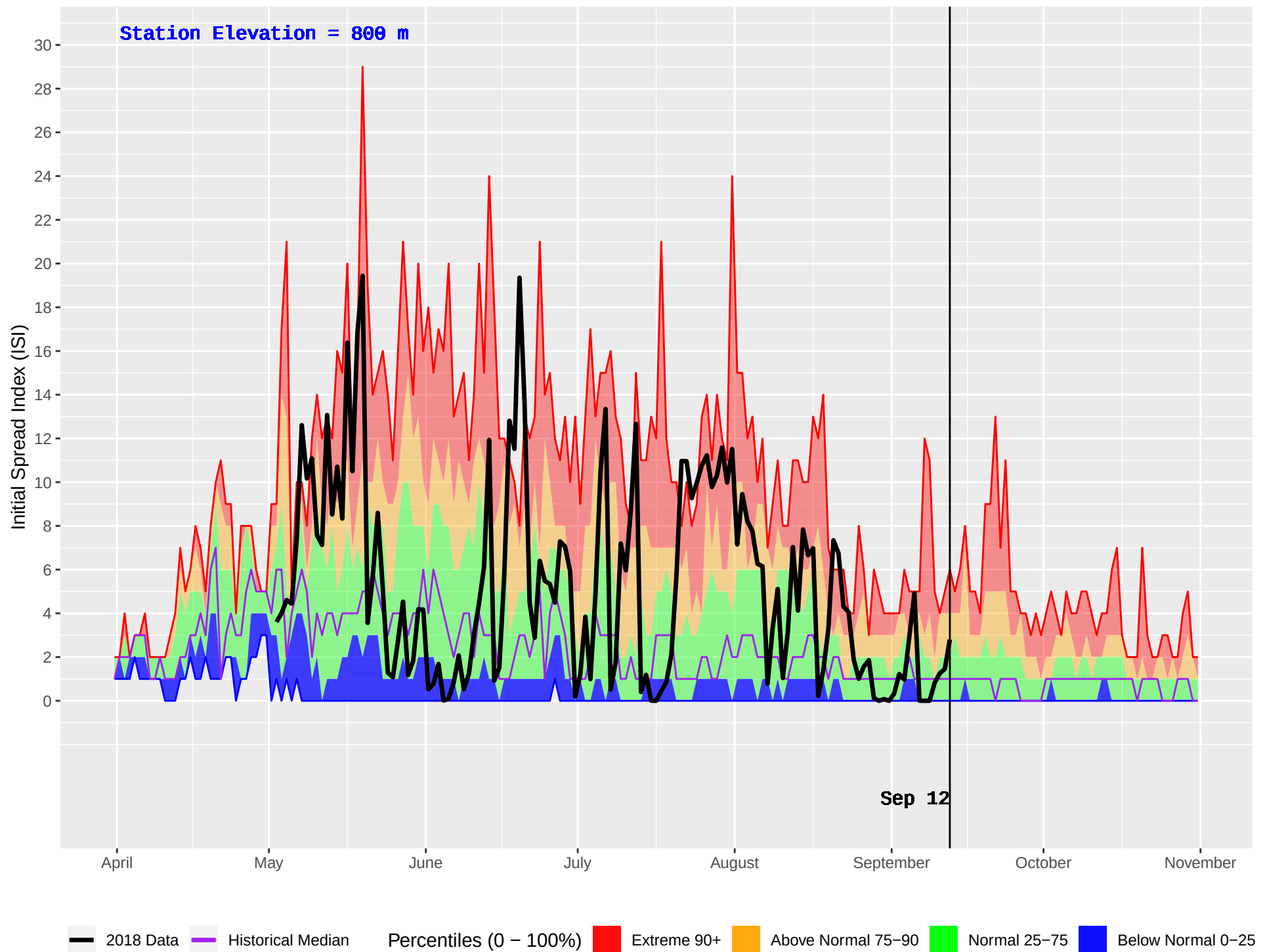
DEASE LAKE FS (108) : Historical (1978–2016) and Current (2018) Daily Initial Spread Index (ISI)
