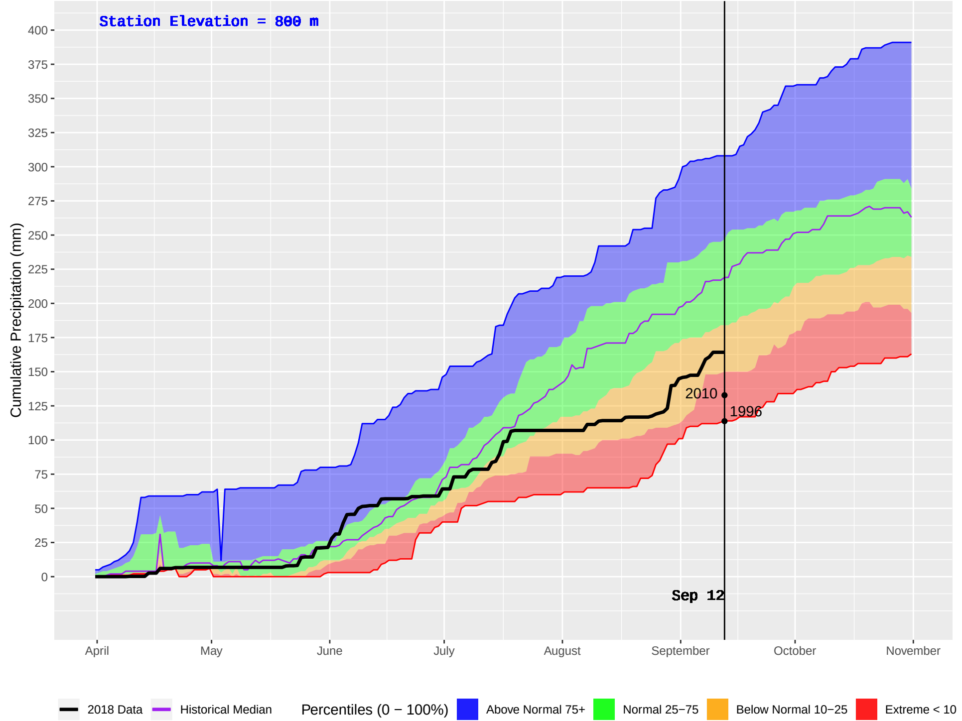
DEASE LAKE FS (108) : Historical (1978–2016) and Current (2018) Daily Cumulative Precipitation
