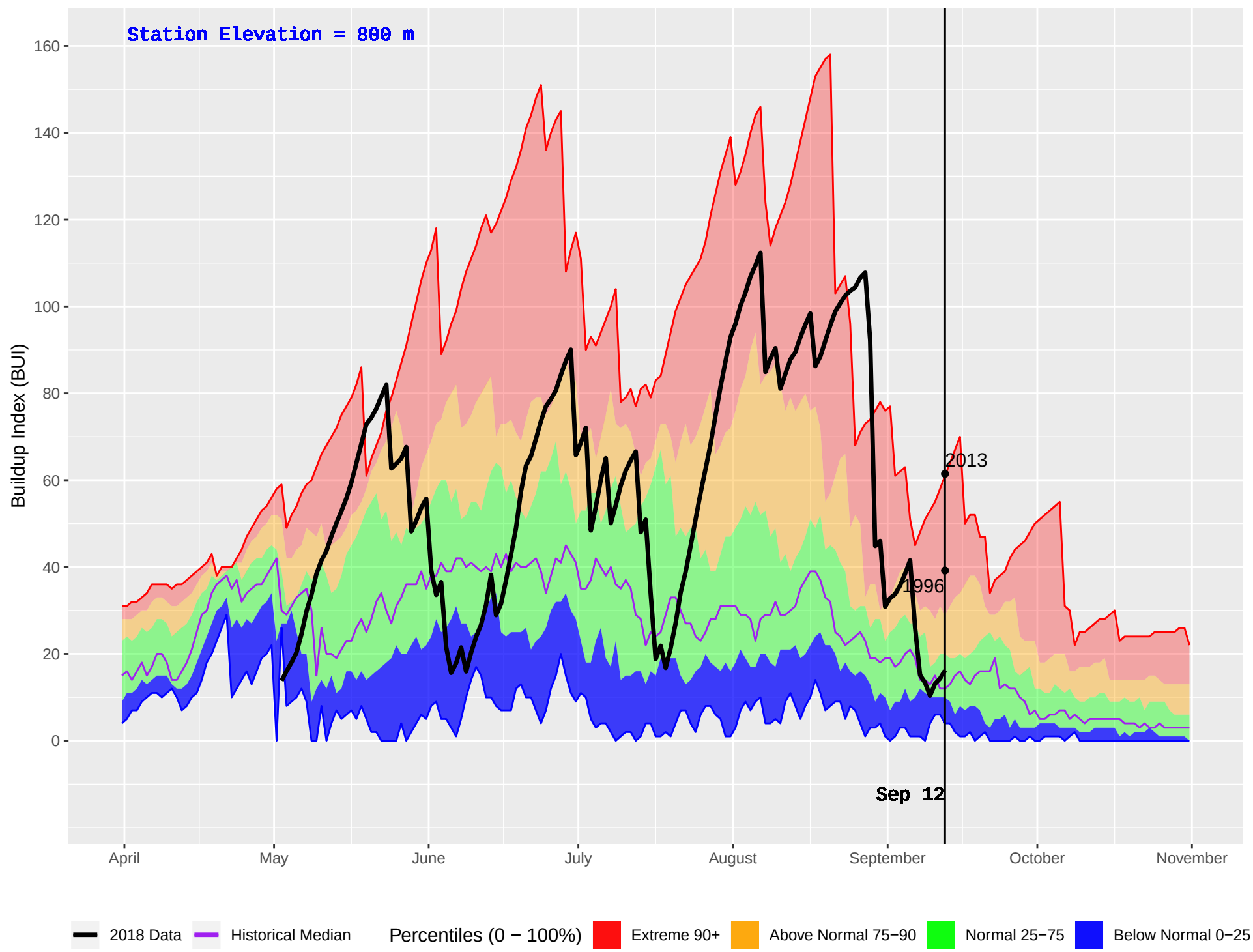
DEASE LAKE FS (108) : Historical (1978–2016) and Current (2018) Daily Buildup Index (BUI)
