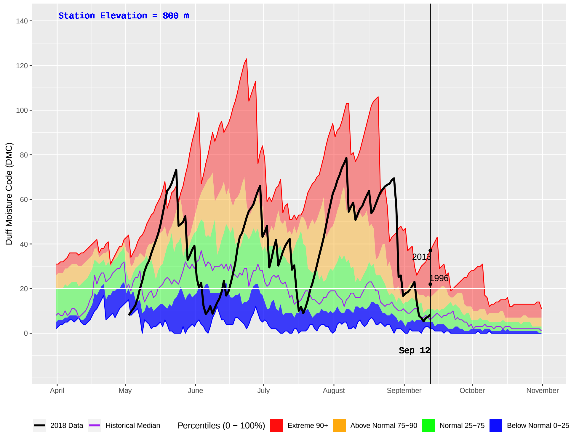
DEASE LAKE FS (108) : Historical (1978–2016) and Current (2018) Daily Duff Moisture Code (DMC)
